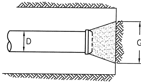
BUTTRESS FOR HORIZONTAL BENDS
