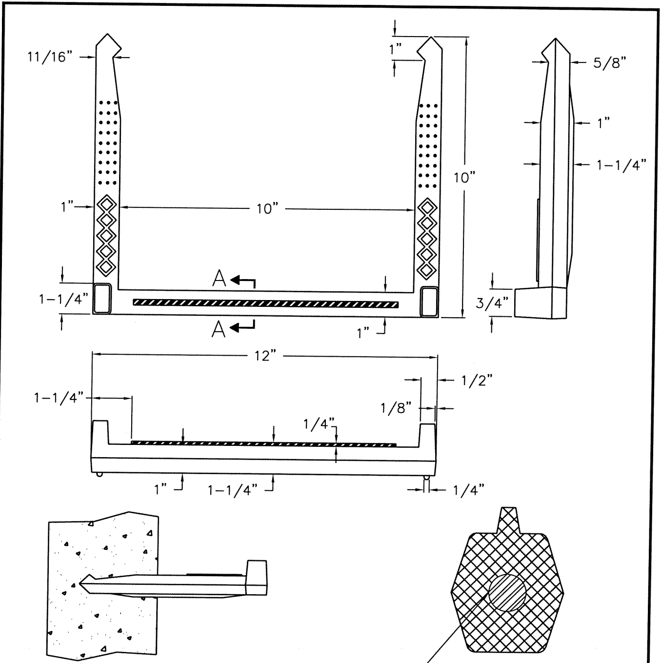
No. 3 Deformed Steel Rod SECTION A~A
